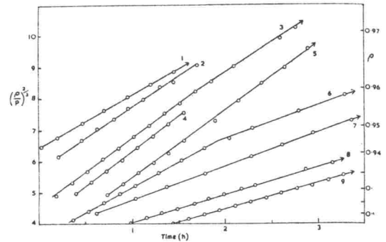
FIGURE 6 Densification data: 9 experiments at 1300°C, pressure 5000 lb.in -2 .
